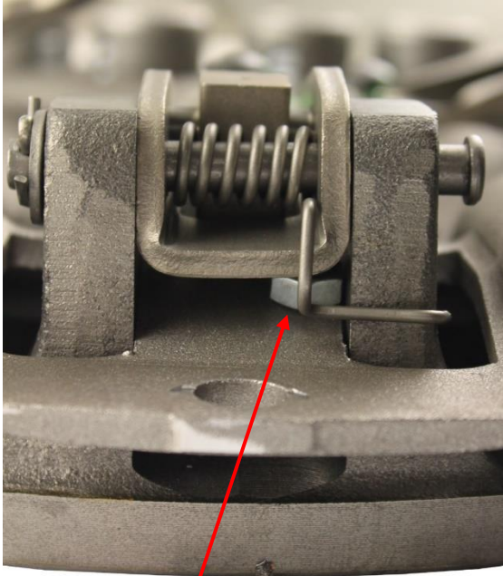
Installation Nut-Remove after Installation of PPA
